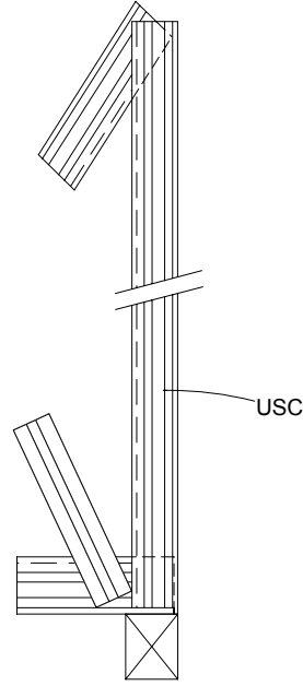
USC End Vertical Detail (End Vertical Expose to Wind)
