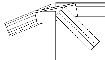
Hip Joint - 2 Webs
