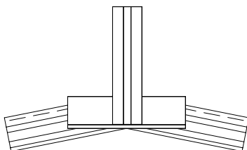
Scissors Bottom Chord Peak- 1 Web
