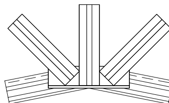
Scissors Bottom Chord Peak- 3 Webs
