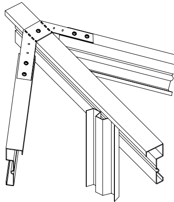
Example Connection Jack to Corner Jack
